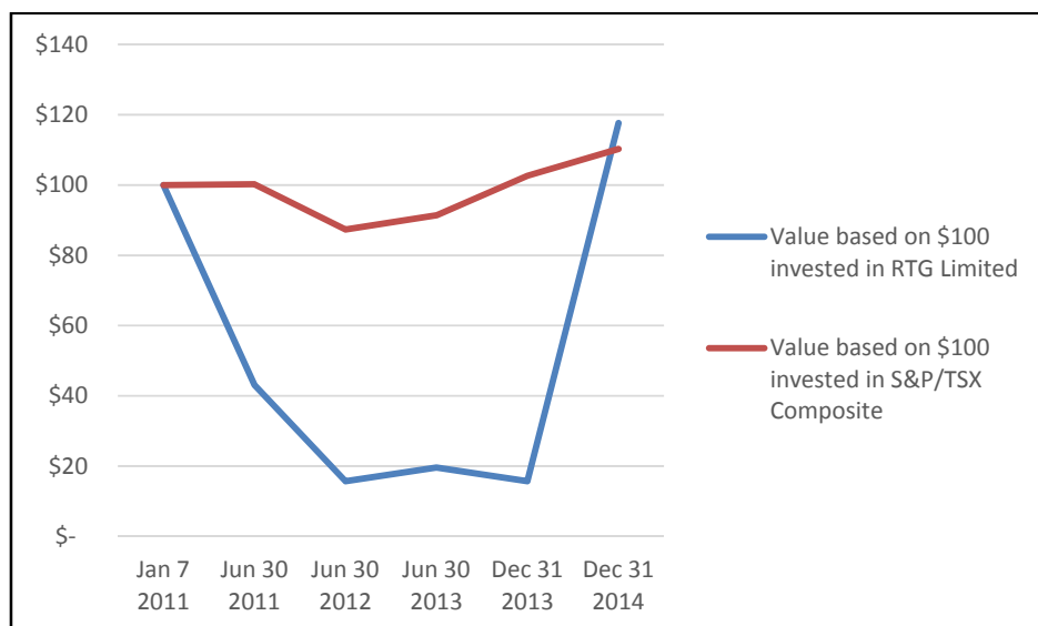
Fig 1 – RTG/TSX S&P Composite Index
